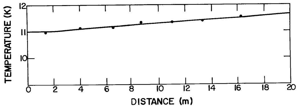
Fig. 4-30. Thermometer location and a typical temperature profile for the Cryenco enclosure.
