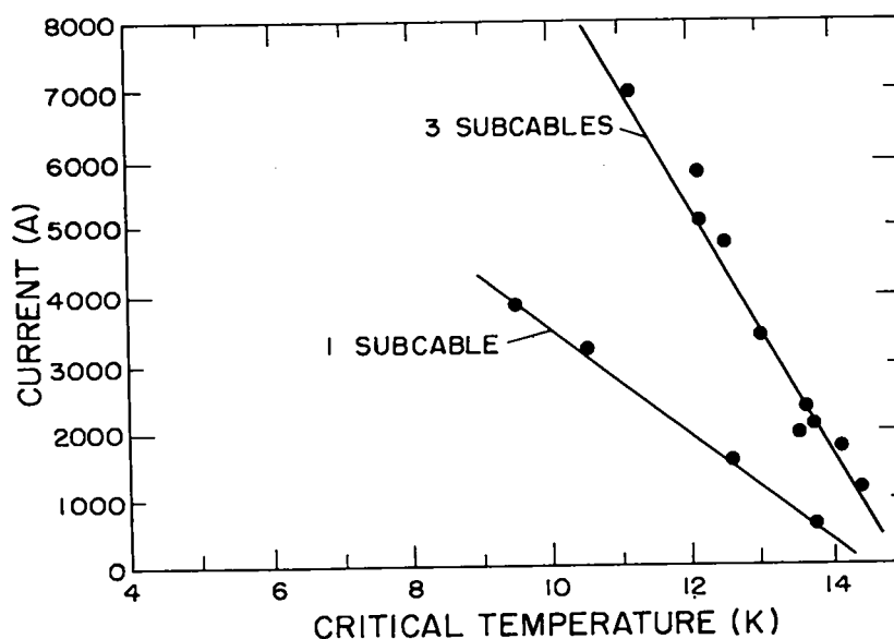
Fig. 4-33. T_c characteristics for Supercon subcables.
