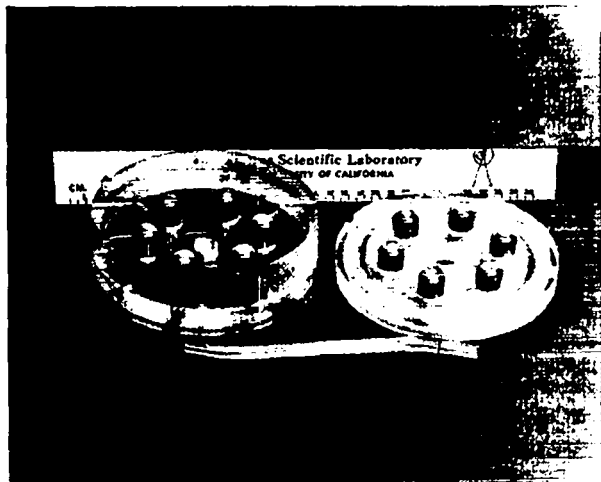
Fig. 3-26. Six-electrode sample holder for multiple breakdown tests.
