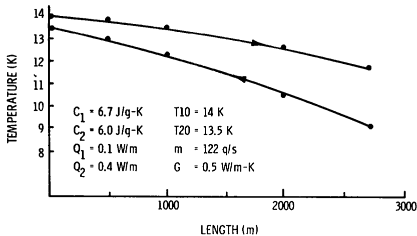
Fig. 4-11. Temperature profile for go and return coolant streams in the model LASL cable with far end expansion.
