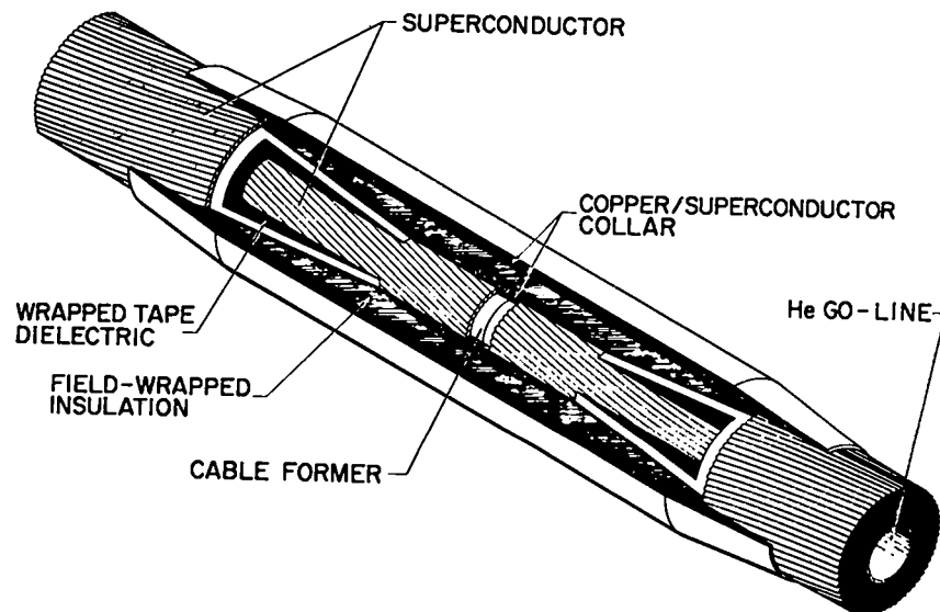
Fig. 5-36. Cable splice design with copper/superconductor connecting collars. Two solder connections are required for each conductor.
