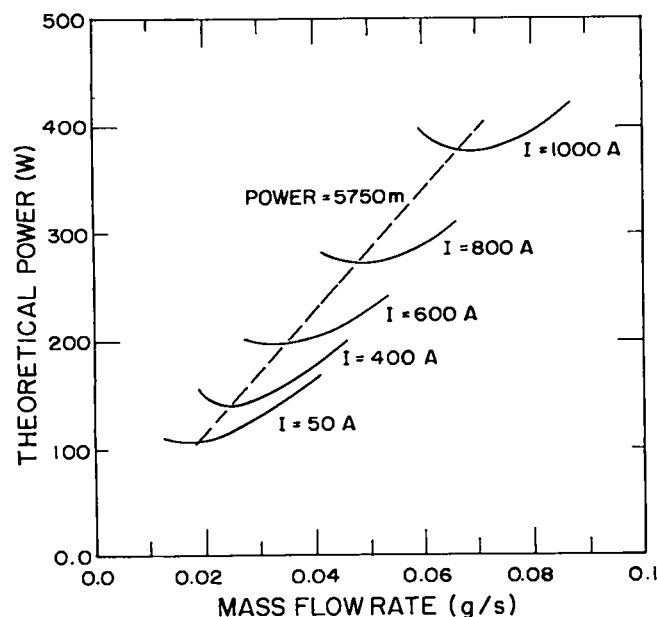
Fig. 4-27. Investigation of optimum performance for a single lead. T_0 = 10 \text{ K} , \ell = 100 \text{ cm} , copper RRR = 100, Biloculine-PTO RRR = 5, solder RRR = 8.
