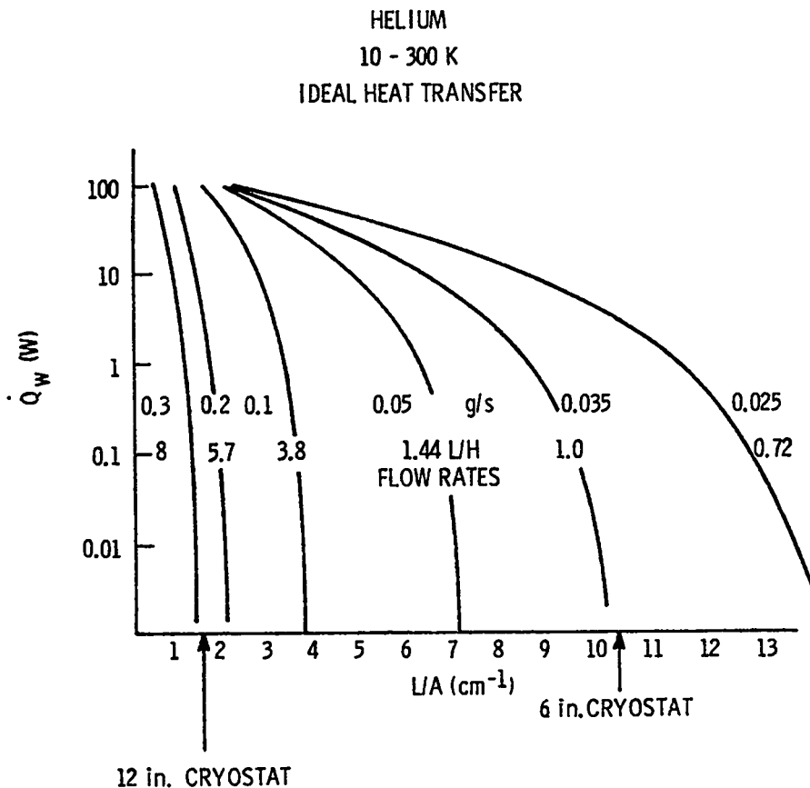
Fig. 4-35. Heat influx down the cooled support tube of the dielectric test cryostat.
