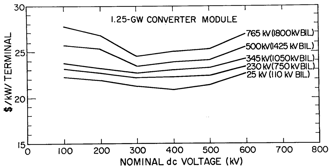
Fig. 6-3. 1.25-GW converter module cost per kW per terminal vs nominal dc voltage for different ac-side voltages.
