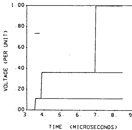
Fig. 3-13. Step response of a semi-infinite, 100-kV, four-conductor dc superconducting cable at x = 1 km. Conductor resistances neglected. R_g = 10 \Omega at x = 0 ; \rho_g = 100 \Omega \cdot m .
