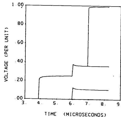
Fig. 3-14. Step response of a semi-infinite, 100-kV, four-conductor dc superconducting cable at x = 1 km. Effect of dielectric constant. R_g = 10 \Omega at x = 0 ; \rho_g = 100 \Omega \cdot m ; k_3 = 3 .
