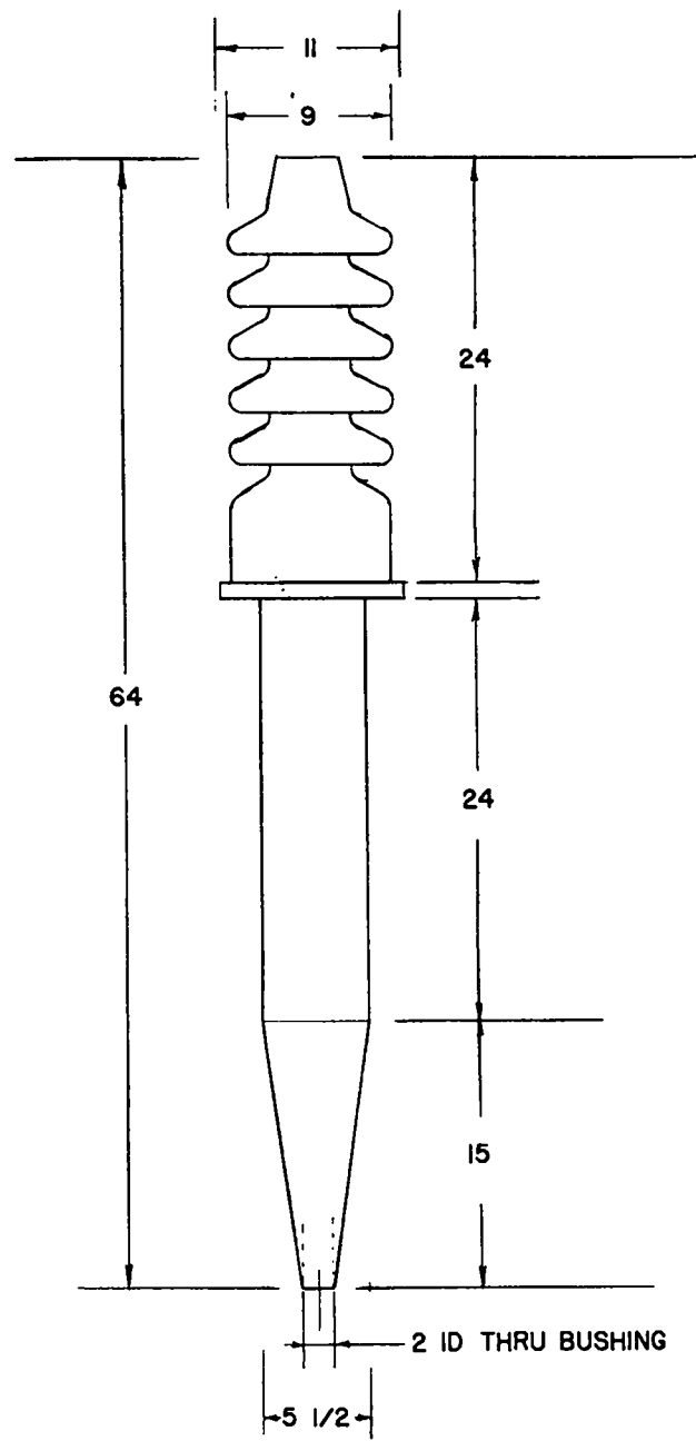
Fig. 3-46. Outline drawing of the second design for the 100-kV epoxy bushing.
