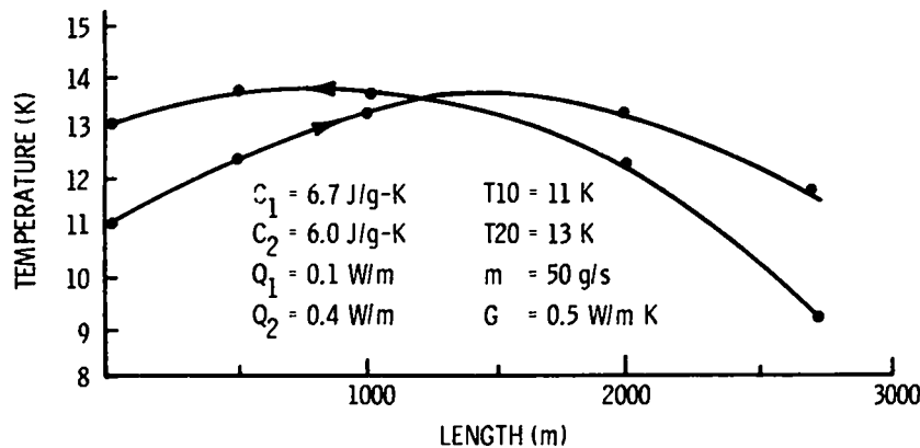
Fig. 4-12. Temperature profile for go and return coolant streams in the model LASL cable with near and far end expansion.
