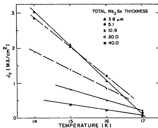
Fig. 5-8. Critical current density as a function of temperature for Nb_3Sn tapes having five different thicknesses.
